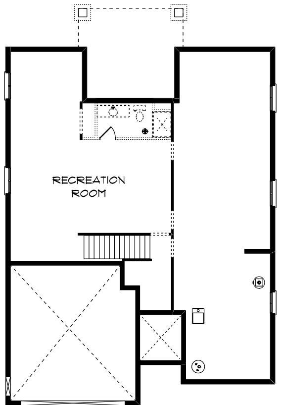
FOUNDATION PLAN
