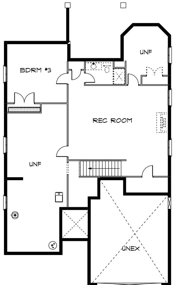
FOUNDATION PLAN
